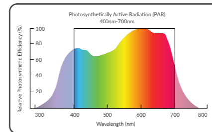
Usable colour spectra for optimal plant growth, measured in-house by Aglo Photometrics utilising LabSpion Goniospectrometer technology.
