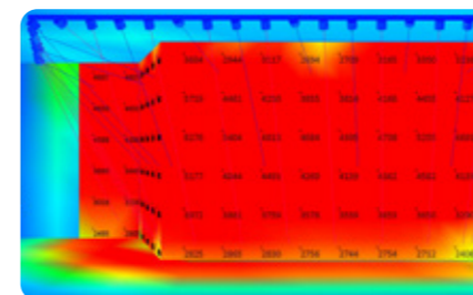
Pseudo-colour render of green wall illuminance distribution.
