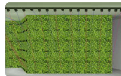
3D render of green wall lighting plan.
