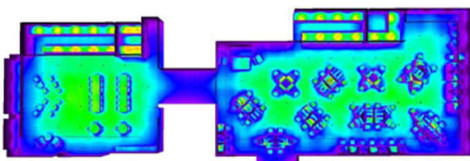
Pakenham Hotel Gaming Room: Lux Map calculations indicate expected illumination levels throughout the site.
