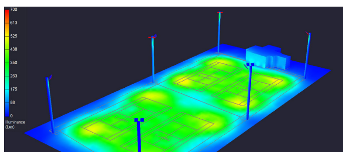
Tennis court lux map
